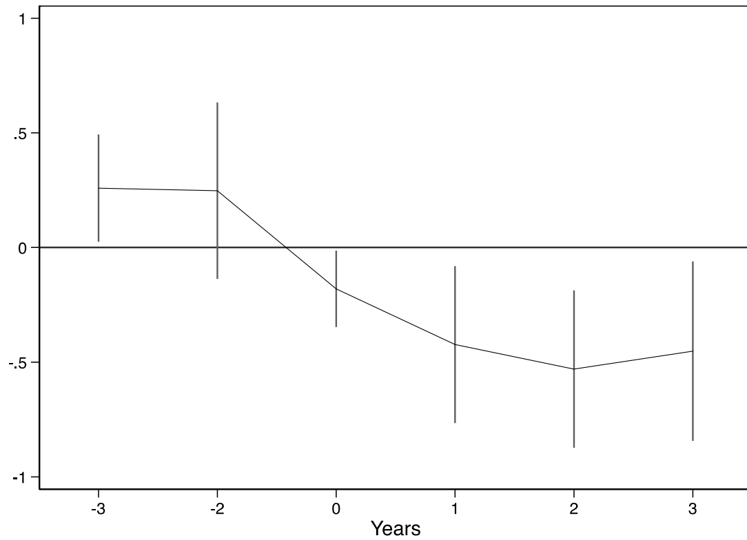
Figure 3: Event Study
