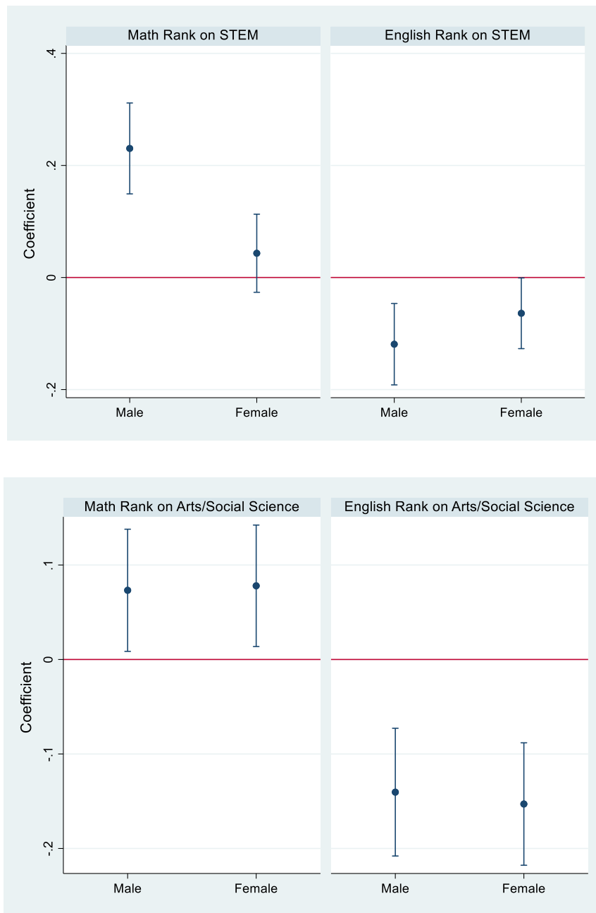
Figure 2: Effect of Rank in Math and English on Field of Study by Gender
