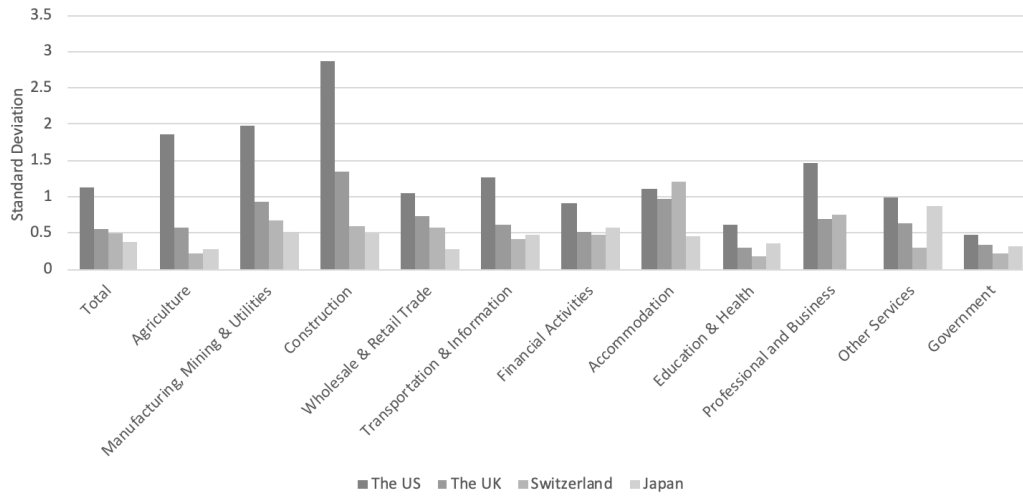
Figure 6: Standard Deviation of Output, \sigma_{\Delta y} , for 11 Sectors
