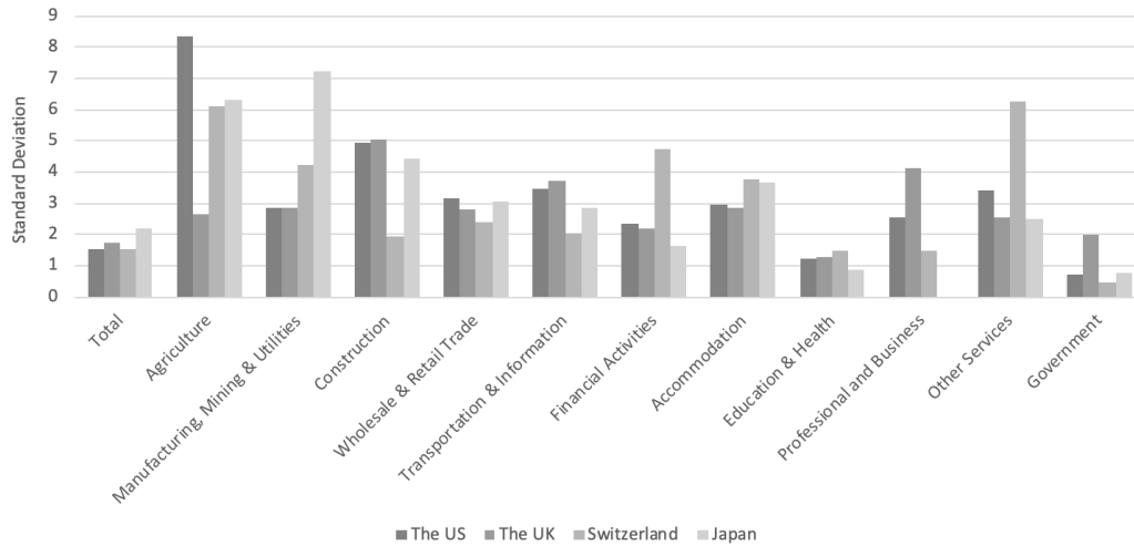
Figure 6: Standard Deviation of Output, \sigma_{\Delta y} , for 11 Sectors
