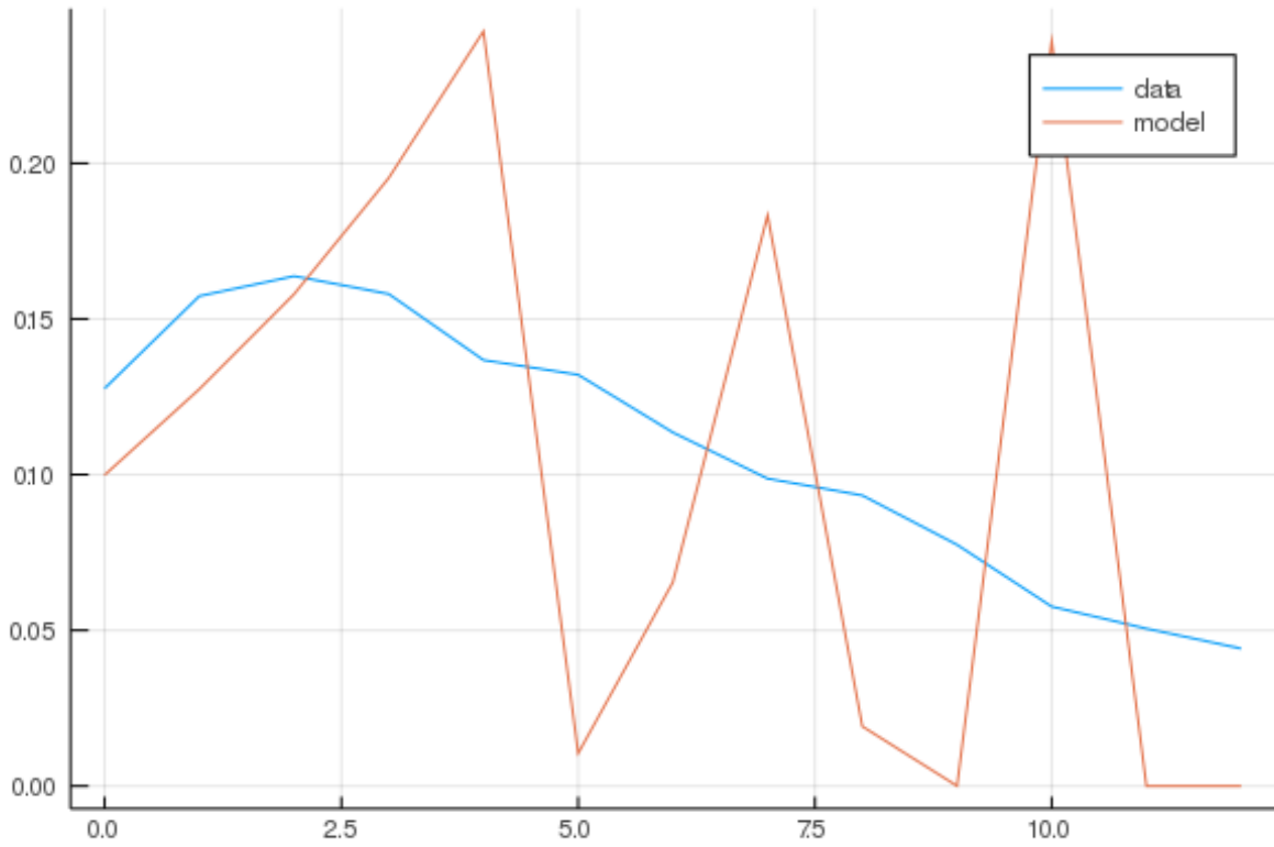
Figure A.4: Model fit: 1(use platform in week t)
