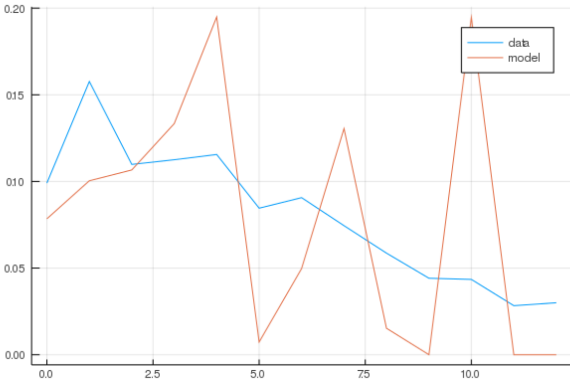
Figure A.5: Model fit: number of inquiries in week t
