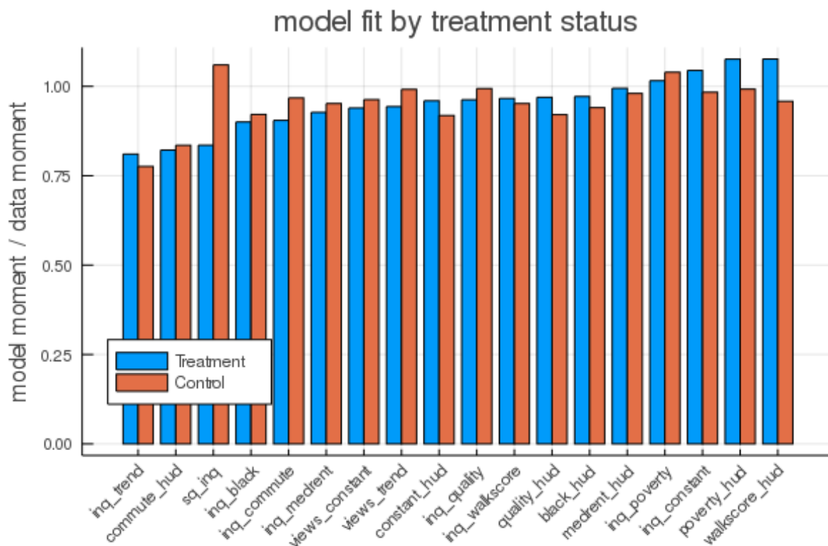
Figure A.3: Model fit: all moments
