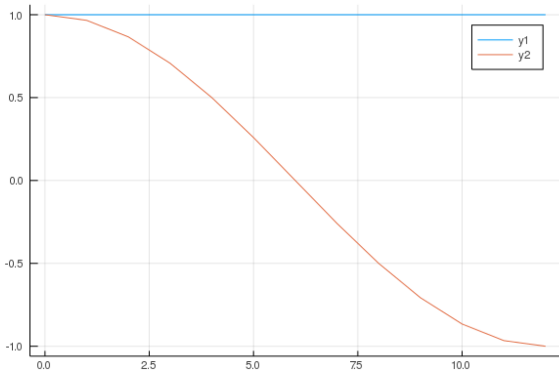
Figure A.2: Basis functions for time-varying moments
