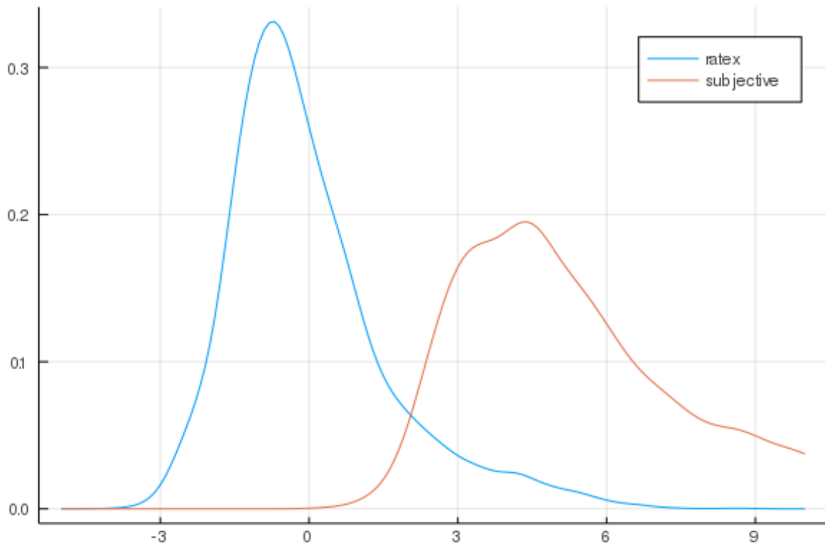
Figure 12: Kernel density of residuals q - E(q|x)
