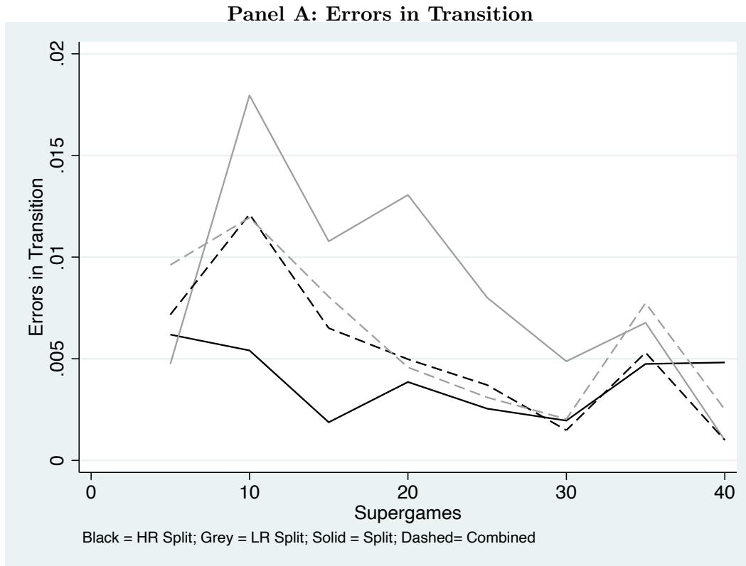
Figure A.3: Errors in transition and action , Error rates across different treatments and groups. The average is computed over observations in successive blocks of five supergames. The grey solid line represent the low-IQ split treatment, the black solid lines the high-IQ split treatment, the dashed lines the combined treatment: grey is the low-IQ group, black is the high-IQ group.
