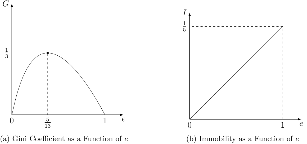
Figure 6: p(\theta) = \sqrt{\theta} .
