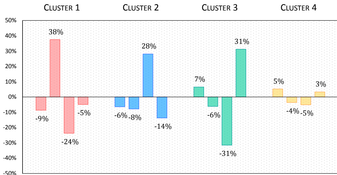
Fig. 2: Subject deviation by cluster in comparison to sample mean
