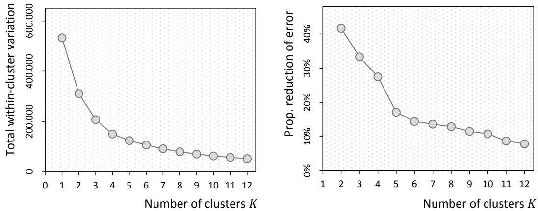
Fig. 1: Total within-cluster variation (left) and proportional reduction of error (right) Notes: Values are averaged over 1 000 replications of K -means with random starting centres.
