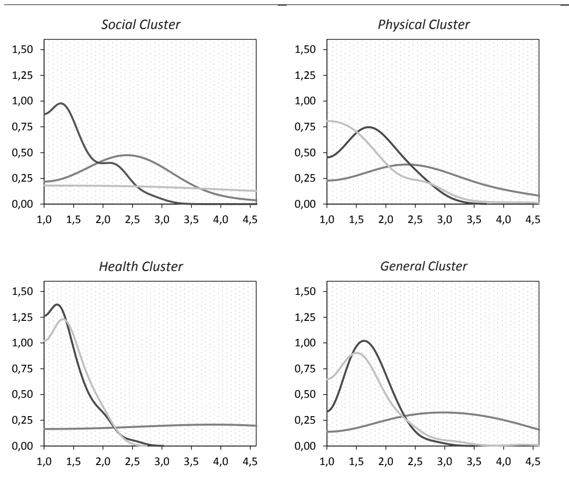
Fig. C.1: Density estimates of bias-corrected efficiency scores by cluster and country Notes: Great Britain (dark), Germany (medium), and Italy (light) are distinguished by greyscale.
