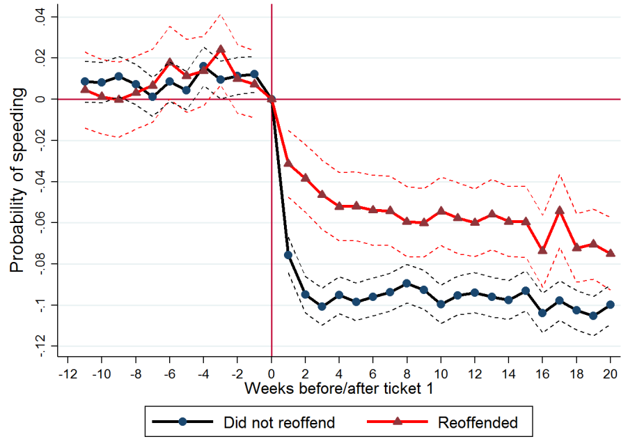
Figure 15: Event study estimates by reoffence pattern
