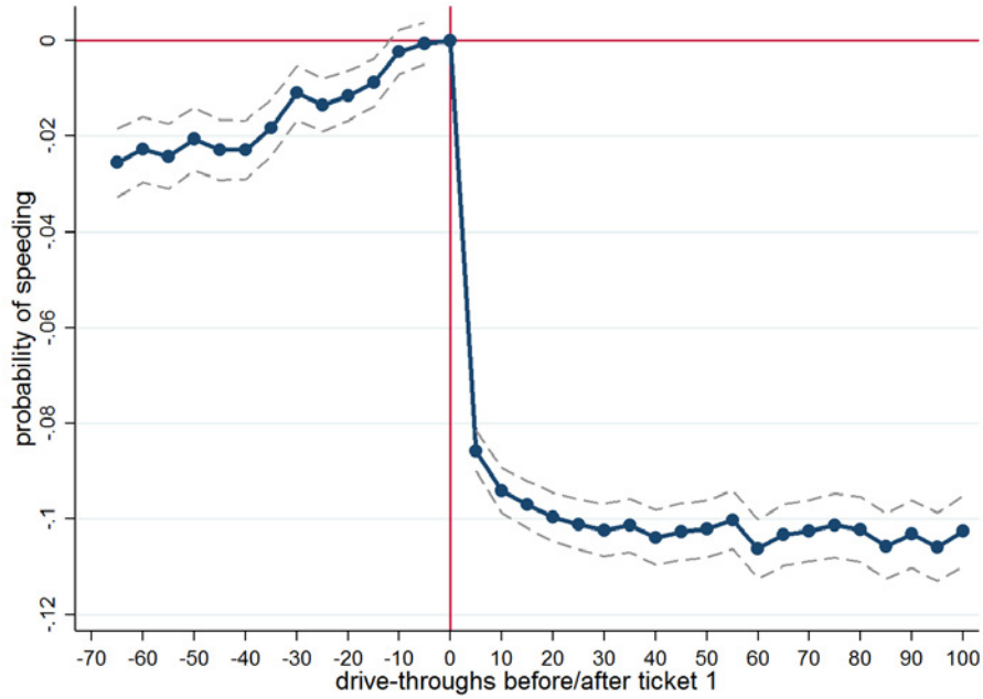
Figure 14: Event study estimates by ride sequence
