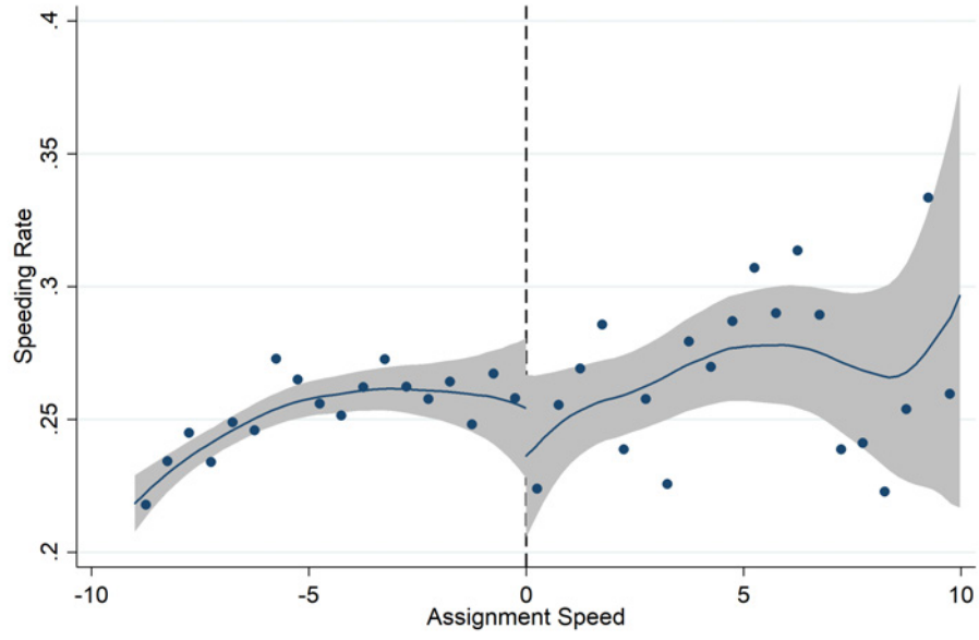
Figure 6: Discontinuities in outcomes at the high-fine cutoff
