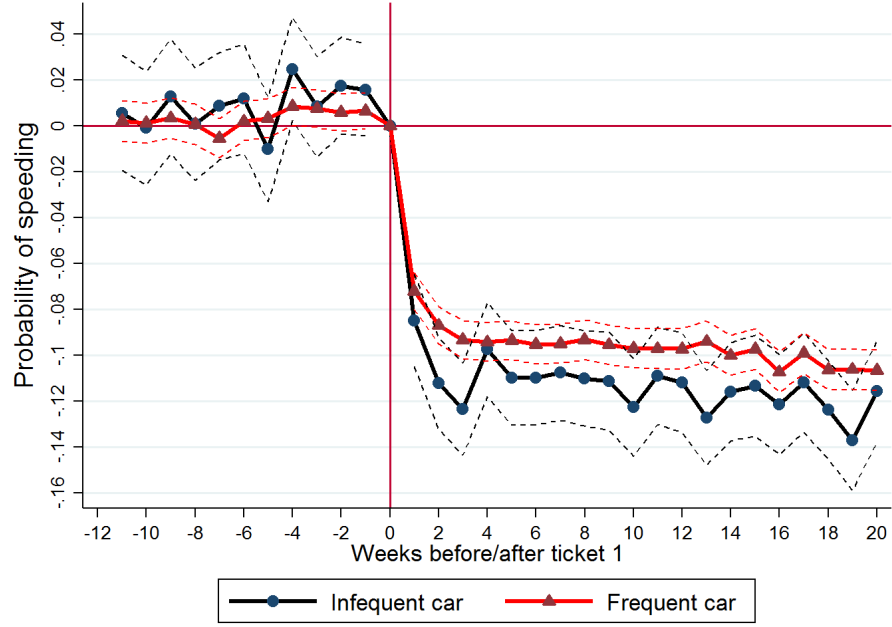
Figure A.16: Heterogeneity: speed and speeding responses by driving frequency (a) Outcome: Speeding
