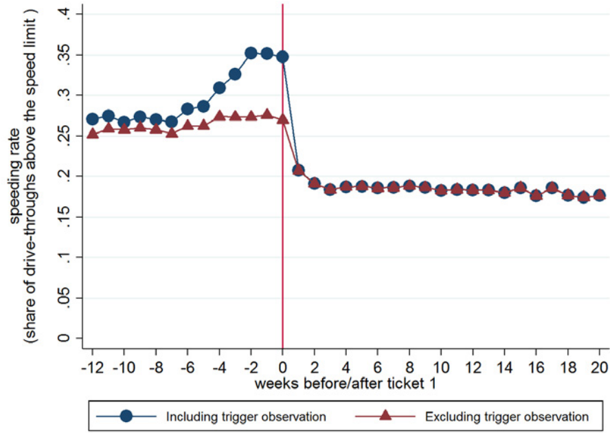
Figure 7: Event study: plot of raw data
