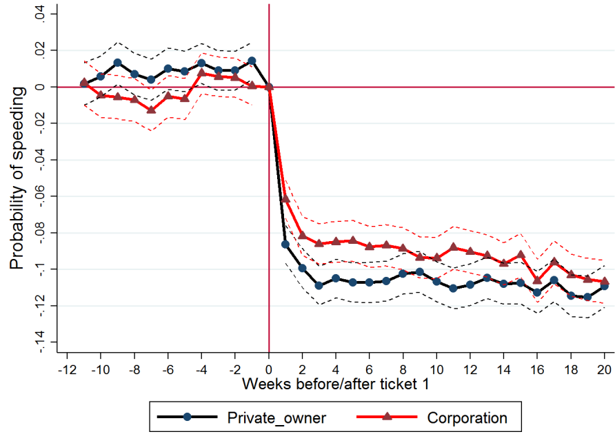
Figure 12: Event study estimates: private owner vs corporation
