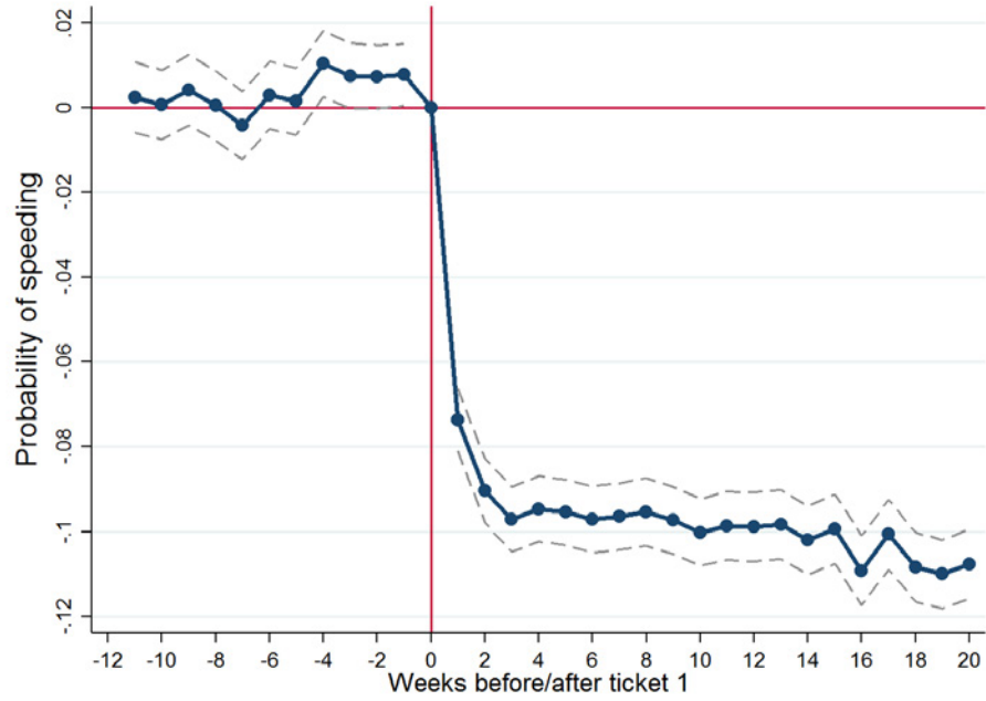
Figure 8: Event study estimates: responses to a low-fine ticket
