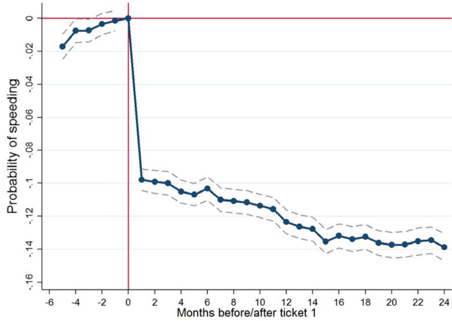
Figure 10: Event study estimates: long-run effects
