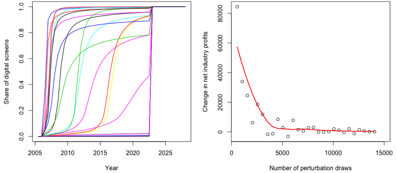
(a) Simulated industry paths (20 perturbation draws) (b) Effect of 500 additional perturbation draws on maximized industry profits
