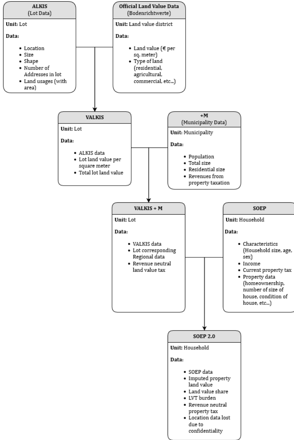
Figure 12: Data flowchart
