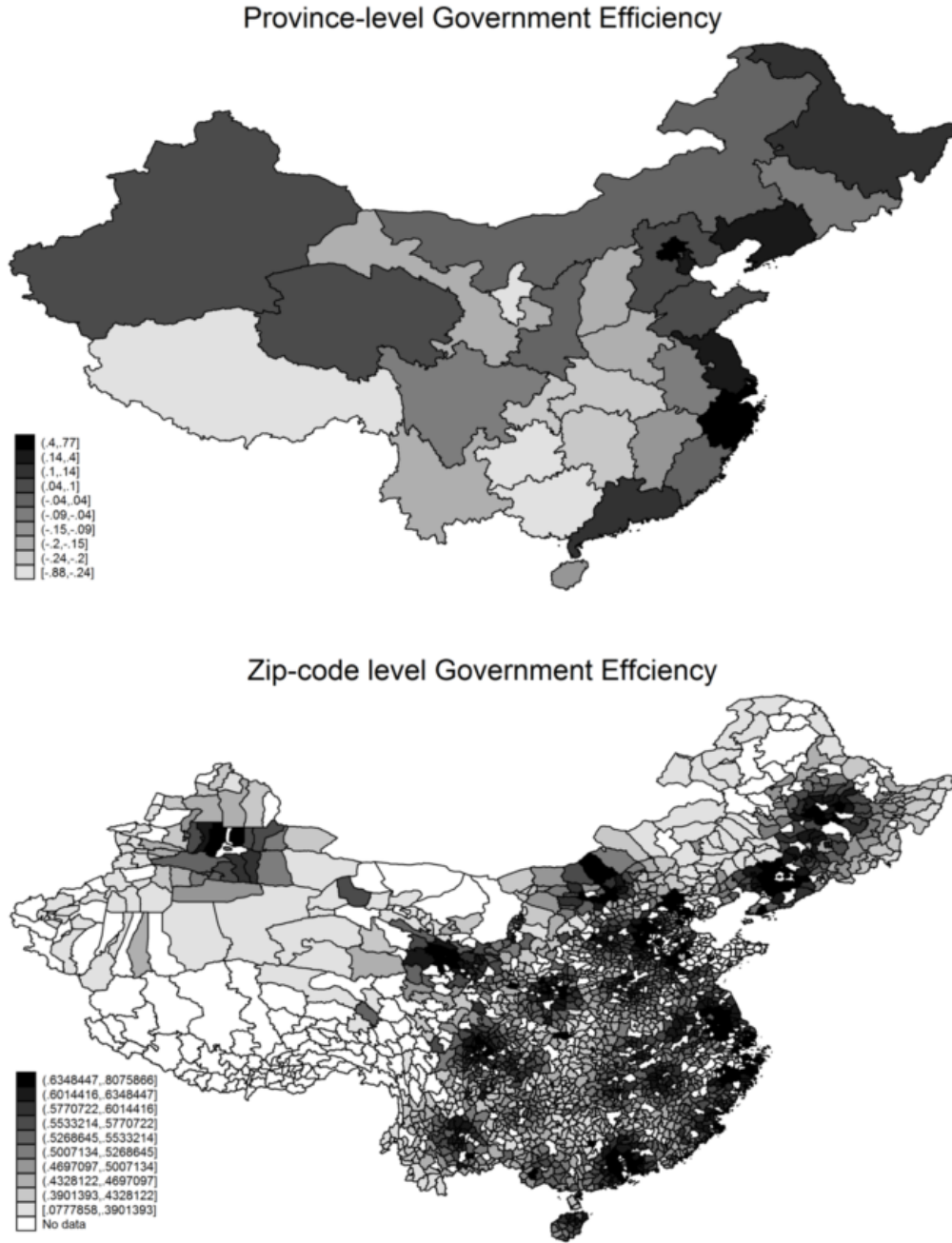
Figure 3: Comparison of province and zip-code level government efficiency
