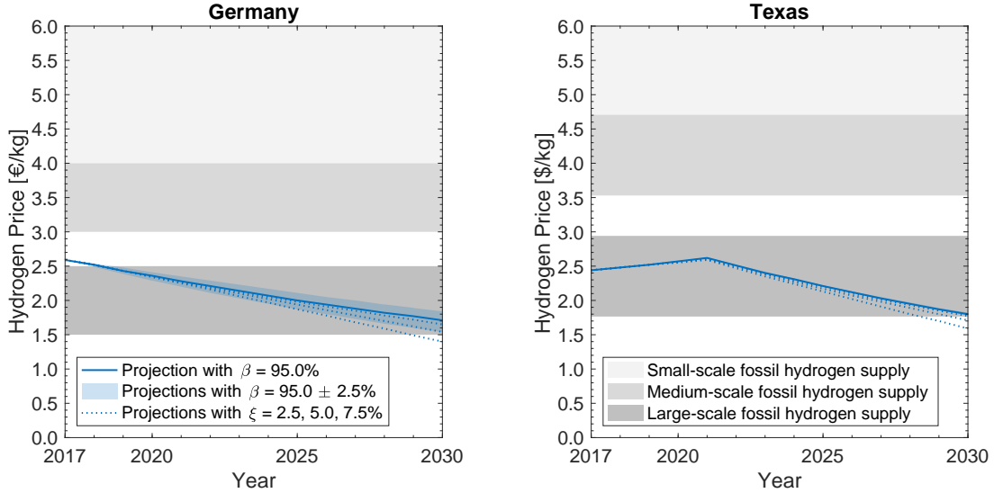
Figure 8: Trajectory of future hydrogen break-even prices.
