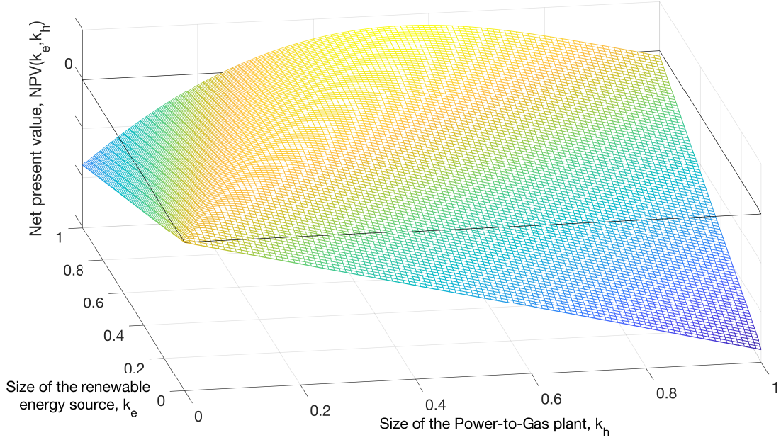
Figure 4: Synergistic investment value for no cost competitive stand-alone energy system.
