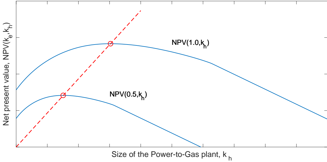
Figure 3: Linearity of the optimal PtG capacity size
