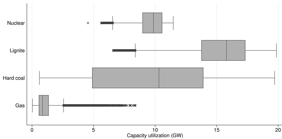
Figure 15: Distribution of power generation by technology
