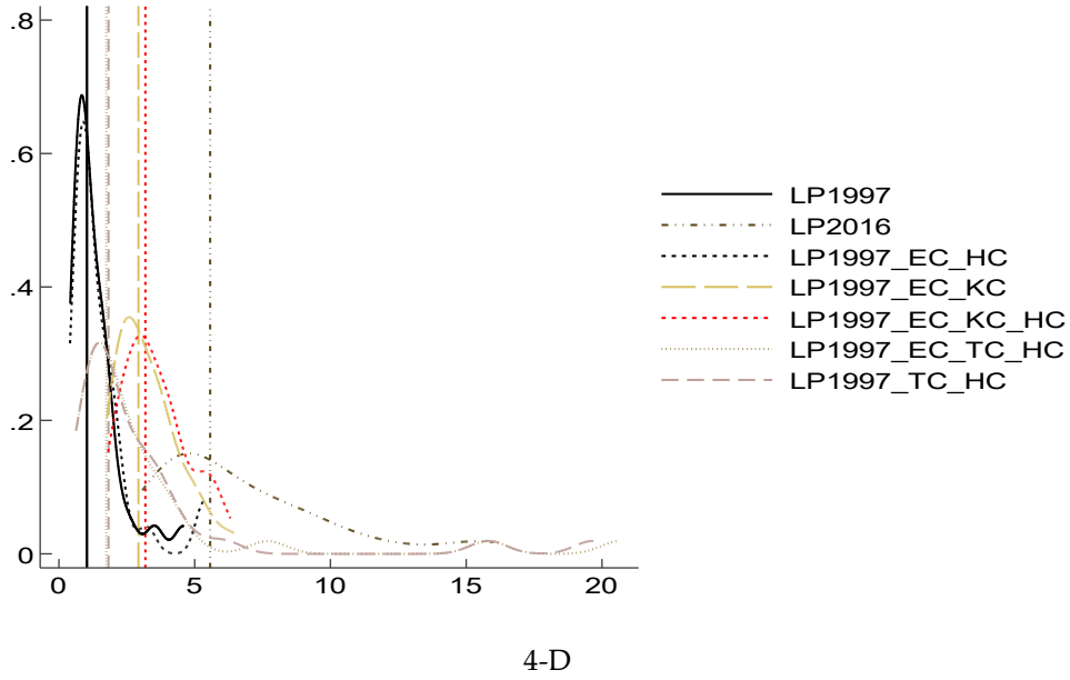
Figure 4: The result of Gaussian kernel density estimation
