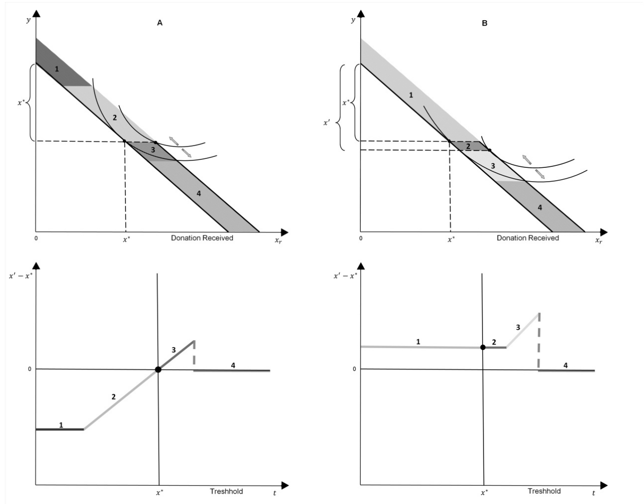
Figure 1: Theoretical predictions
