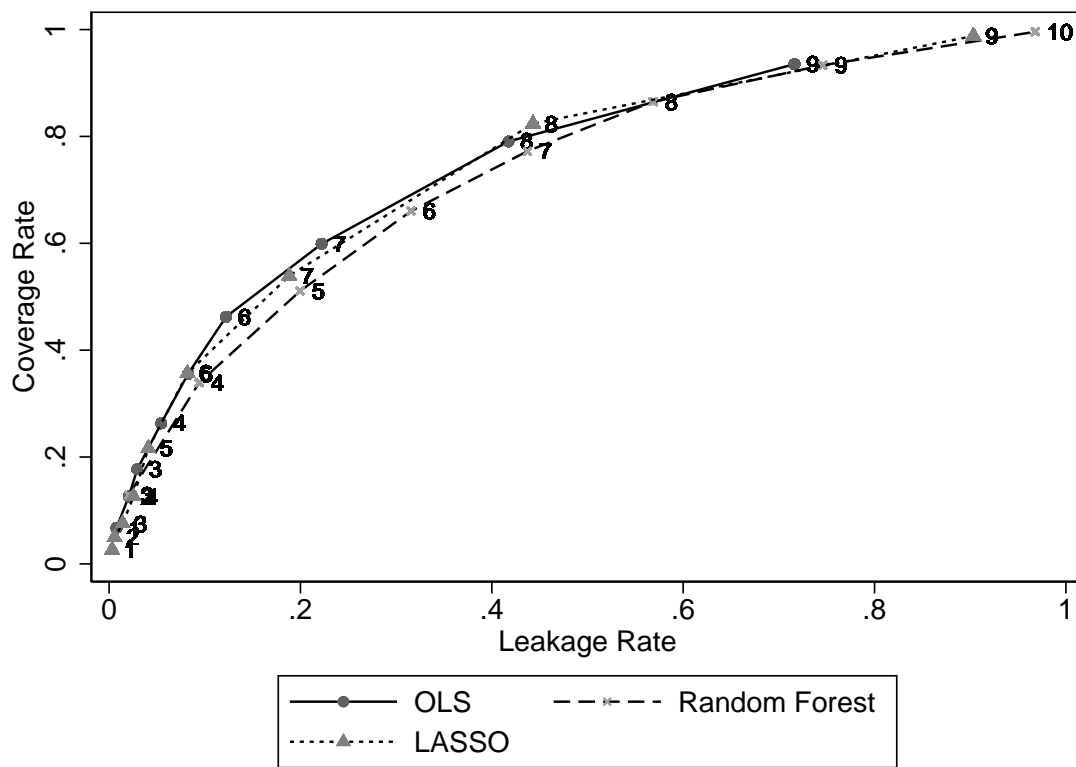
Figure 1: Models' Comparison (Continuous Dep. Var.)
