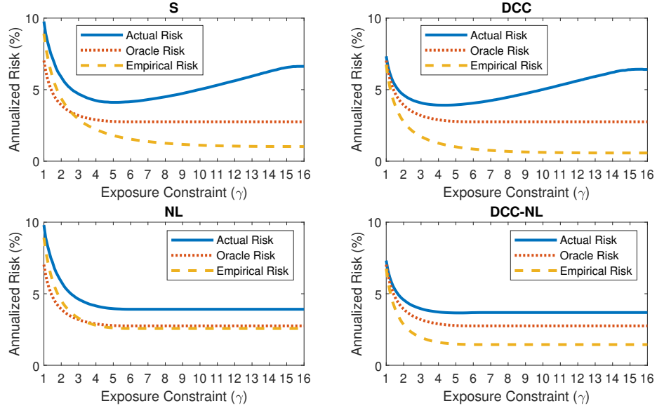
Figure 2: Comparisons of the oracle risks, the average actual risks, and the average empirical risks of the 100 simulated GMV portfolios constructed based on different covariance matrix estimators (S, NL, DCC, DCC-NL) and facing various degrees of leverage constraints (the intensity of the constraint declines with the increase of parameter \gamma ). N = 1000 , and the disturbance terms are drawn from a multivariate standard normal distribution.
