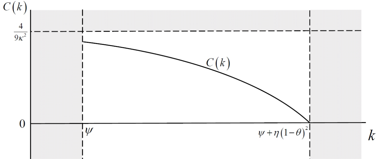
Figure A.1 Properties of the decision rule if \lambda - \theta \geq 0
