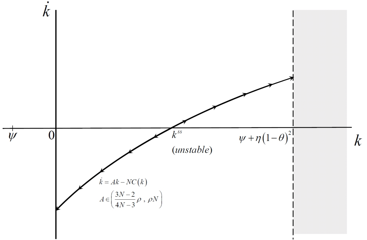
Figure A.3 Resource dynamics in the case where A is such that \psi < 0 .
