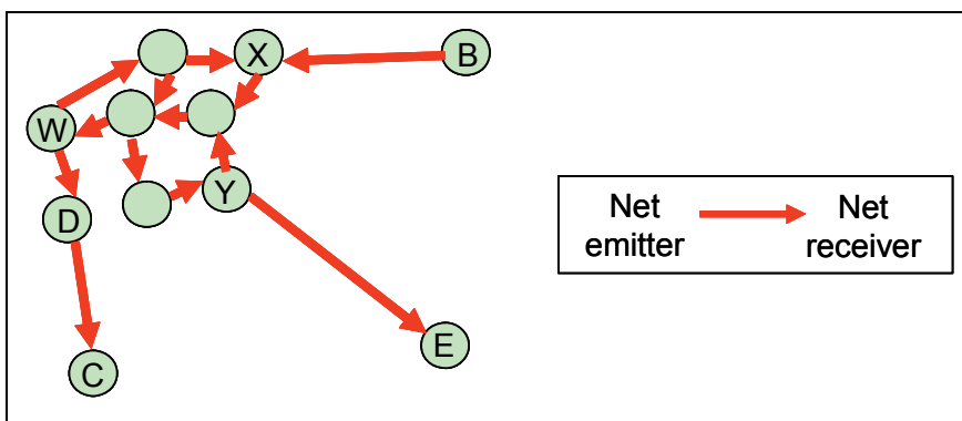
Figure 3.3 Pre-conditioning algorithm
