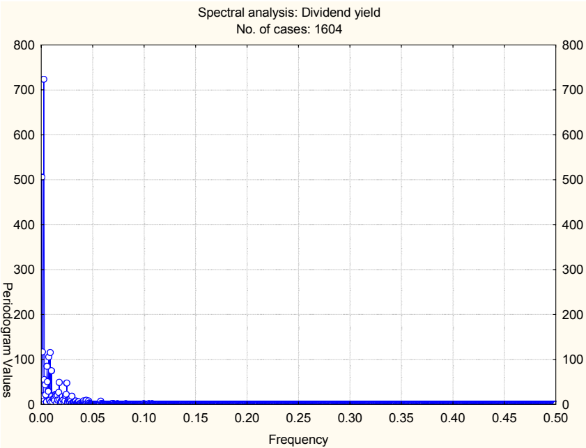
Figure 3.6 Periodogram of dividend yields from Finland 1971–2004, lag = 20
