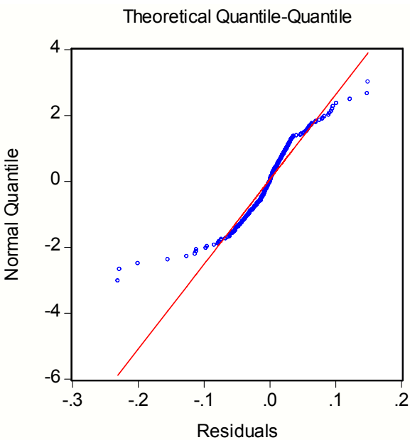
Theoretical quantile-quantile for residuals, Finland
