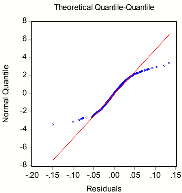
Theoretical quantile-quantile for residuals, United States
