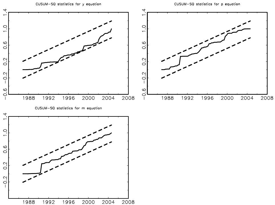
CUSUM of squares test, model with money, 5% significance level.
