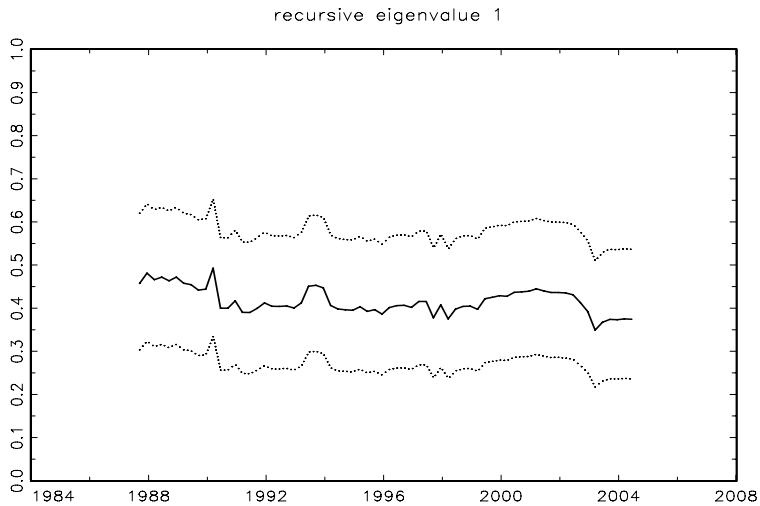
Figure: Recursive eigenvalue analysis of the VEC model for real broadly defined liquidity.
