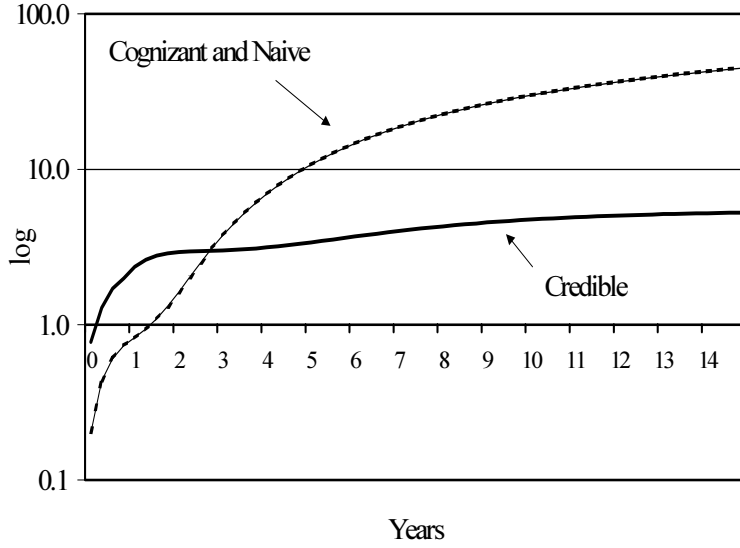
Figure 4.4 Cumulative quadratic loss \frac{1}{2}*(\text{infy}-\text{inf})^2 + \frac{1}{2}*(U-\text{NAIRU})^2
