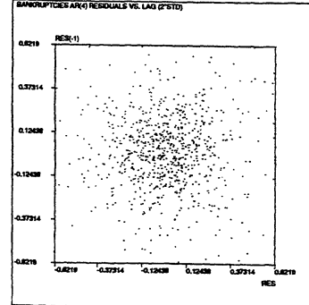
Figure 5. Two-dimensional plots of AR(4) residuals
