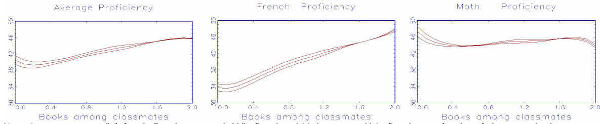
Figure 4.2: Expected achievement E[Y^{b,c}] in rural areas
