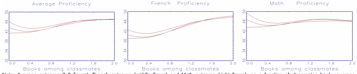
Figure 4.1: Expected achievement E[Y^{b,c}] as a function of own books and classmates book coverage
