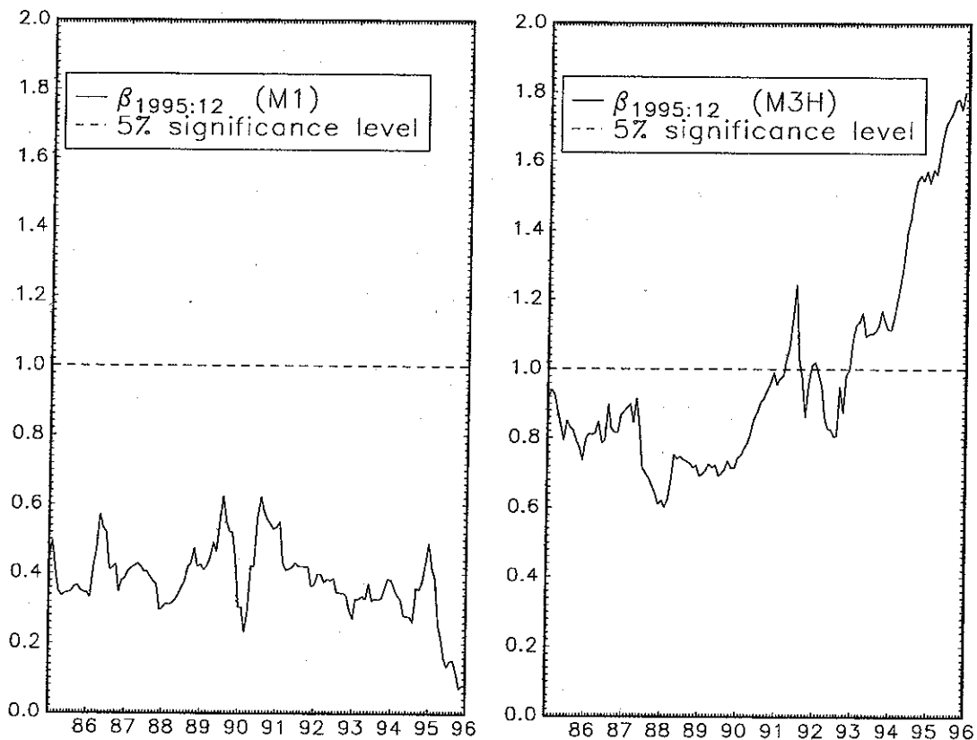
Figure 3.2 Recursive Tests for Restricted \hat{\beta}_{1995:12} \in \text{sp}(\hat{\beta}_\tau) , \tau = 1985 : 1, \dots, 1995 : 12
