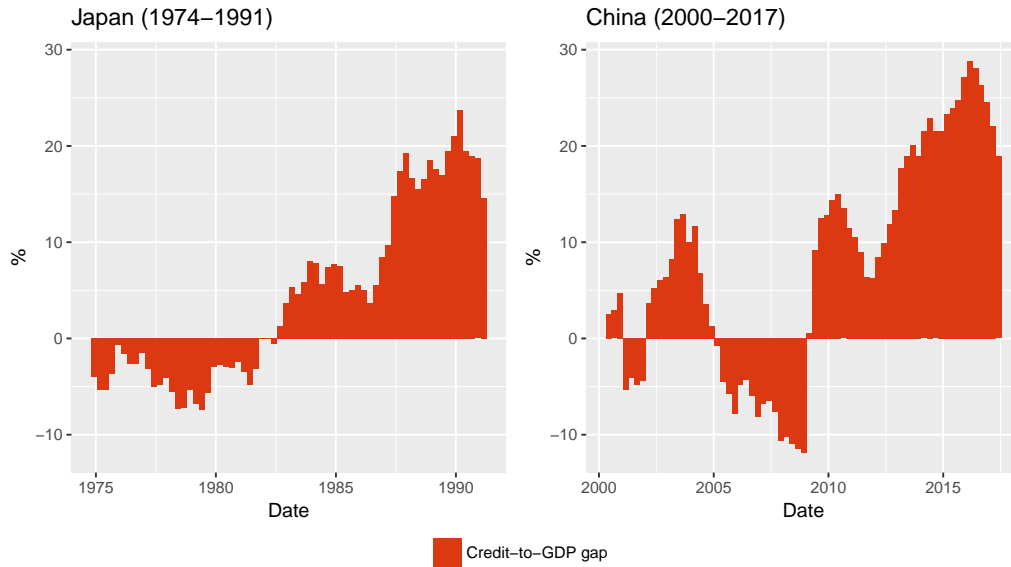
Figure 16: Credit-to-GDP gaps
