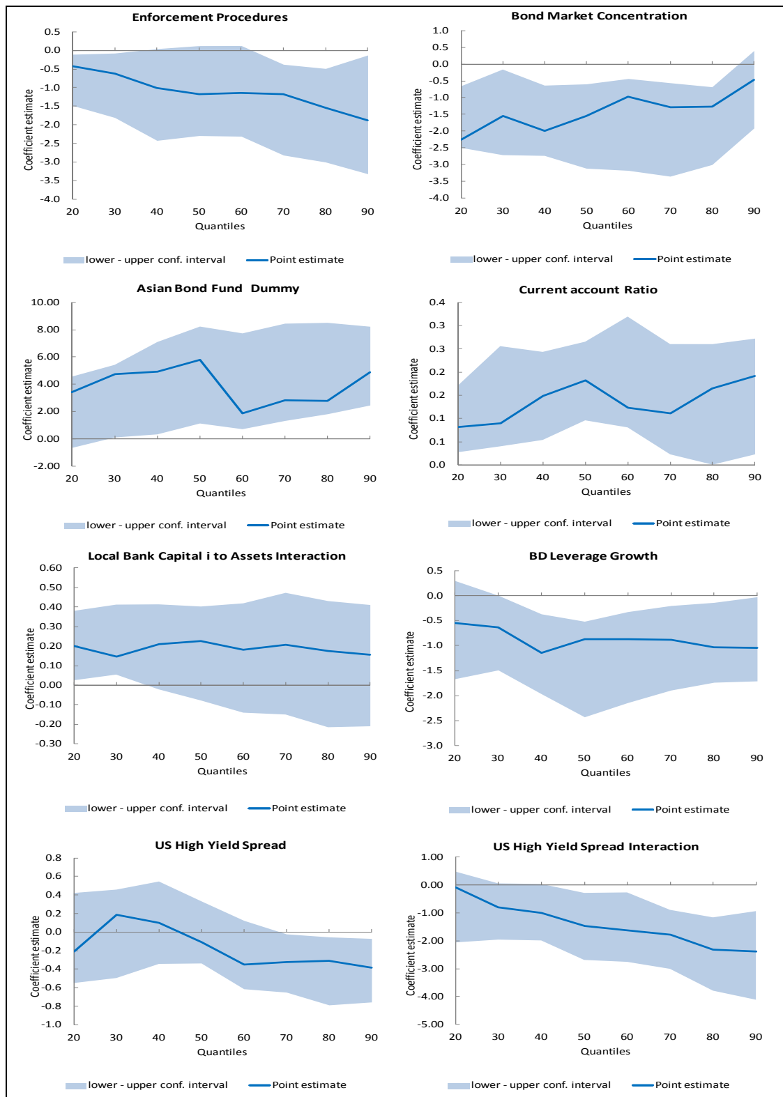
Figure 7 Quantile regression results: Dropping insignificant regressors
