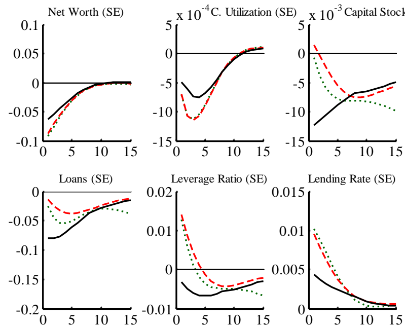
Figure 7 Impulse responses of low-risk firm variables to a 1% increase in the policy rate
