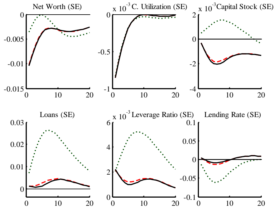
Figure 10 Impulse responses of low-risk firm variables to a positive technology shock
