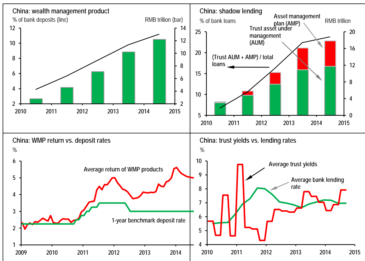
Figure 3 China's shadow banking exposure
