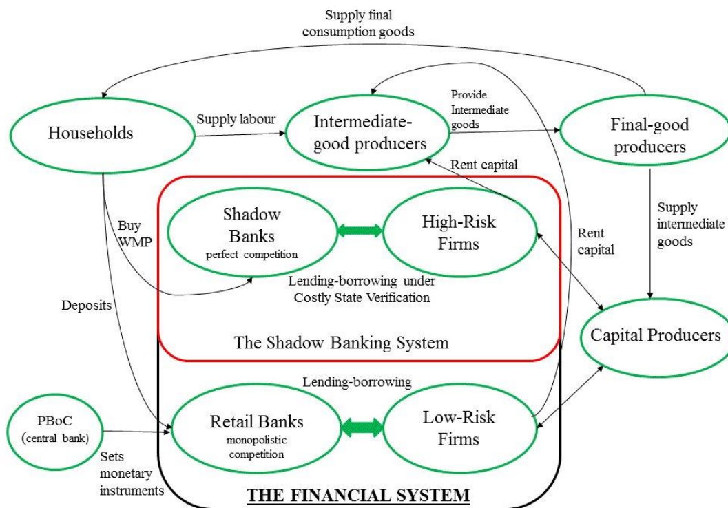
Figure 4 Structure of the DSGE model
