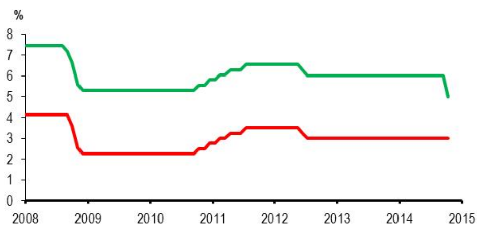
Figure 1 One-year benchmark deposit and lending rates in %: January 2008 – September 2014
