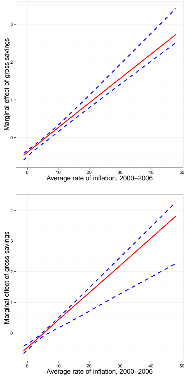
Figure 3: Posterior distribution of the marginal effects of gross savings. The figure is based on the posterior means of the 1000 models with the highest posterior model probability that included all three variables that compose the marginal effect (194, 189). The solid (red) line corresponds to the median and the dotted (blue) lines to the 5th and 95th percentiles. The top figure shows the marginal effect of gross savings on EMPU_{max} , and the bottom figure shows that on EMPU_{max.0006} . All effects are conditional on the average pre-crisis inflation rate.
