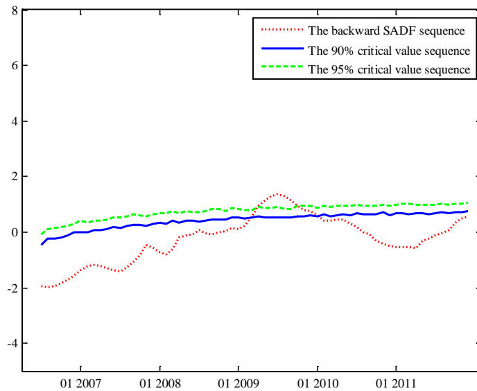
Figure 7 Recursive calculation of the GSADF test for r_0 = 0.4
