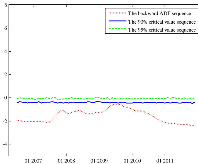
Figure 5 Recursive calculation of the SADF test for r_0 = 0.4
