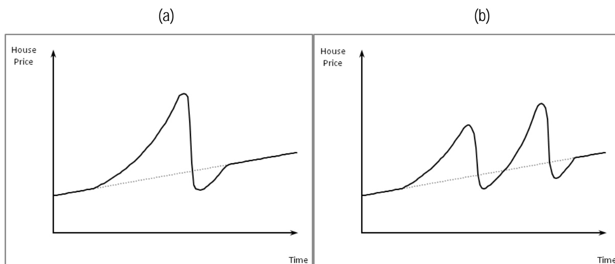
Figure 1 Stylized one-off bubble vs periodically collapsing bubbles
