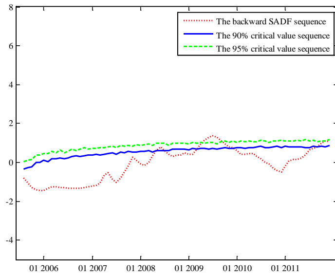
Figure 6 Recursive calculation of the GSADF test for r_0 = 0.3
