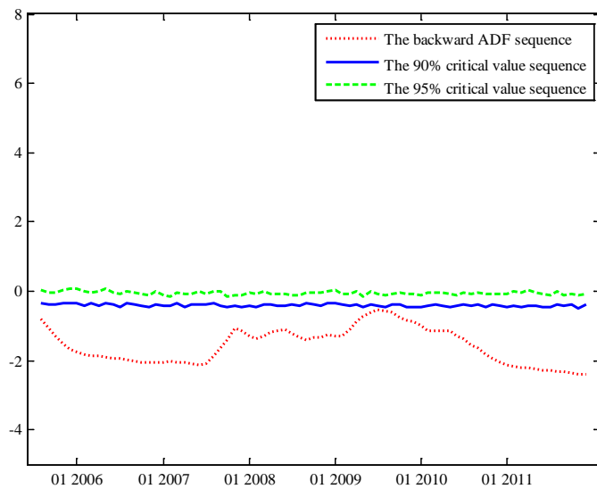
Figure 4 Recursive calculation of the SADF test for r_0 = 0.3
