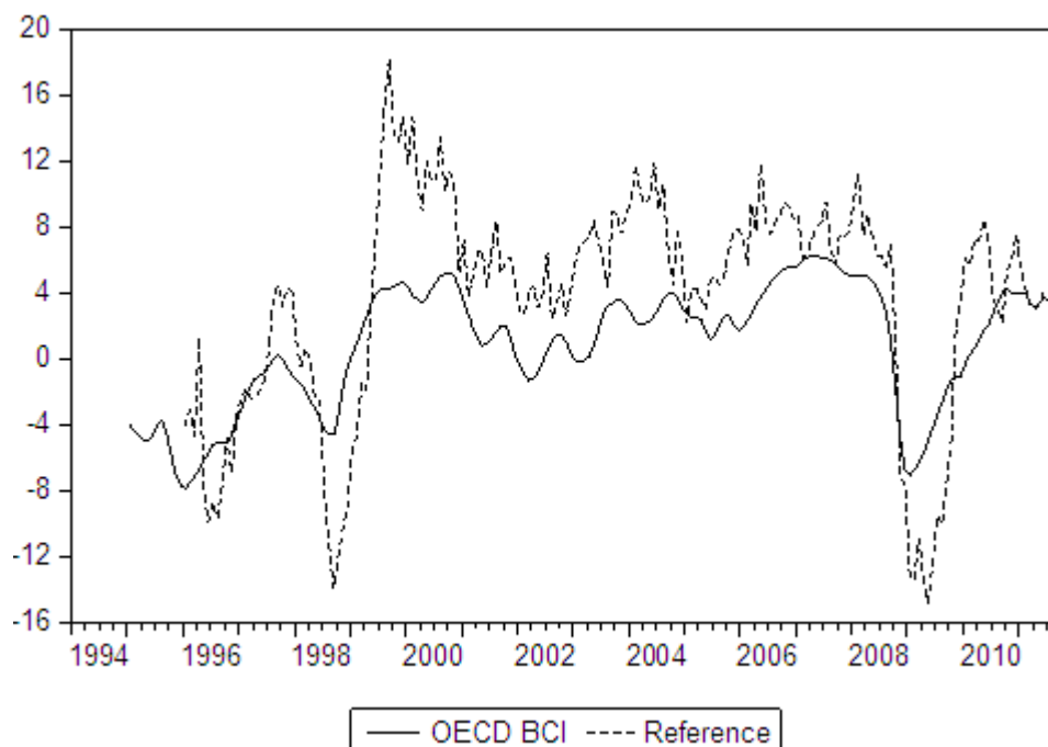
Figure 6 Reference series plotted against OECD BCI.
