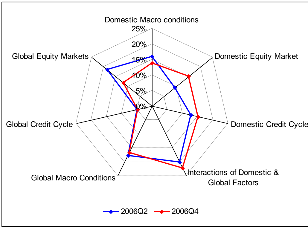
Figure 4 Predicting the 2008/2009 financial crisis in the United States. Factors contributing to systemic risk (% share) in 2006q2 and 2006q4
