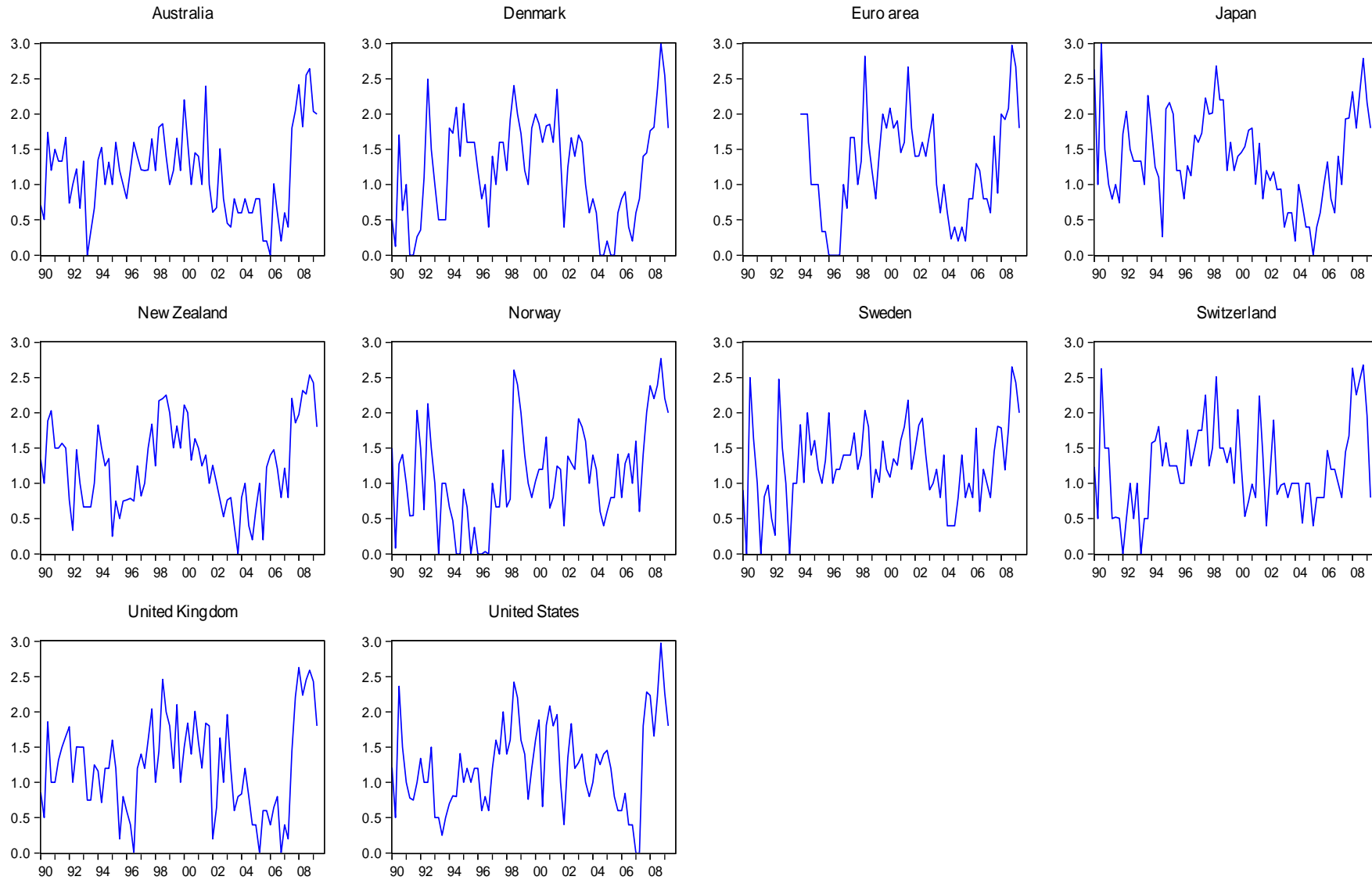
Figure A2 Financial Stress Index for advanced economies in the sample
