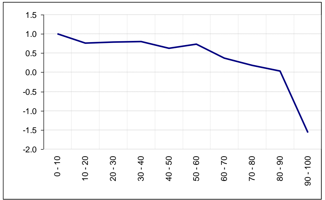
Figure 1 Level of the financial stress index at quarter t and deviation of real GDP from trend at quarter t+2
