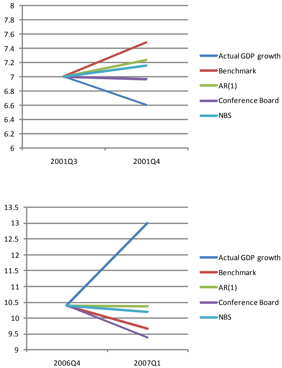
Figure 4. One-step ahead forecasts for 2001Q4 (top) and 2007Q1 (bottom).
