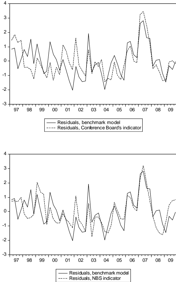
Figure 3. Residuals from benchmark model, together with regressions with Conference Board's coincident indicator (above) and NBS's coincident index (below)
