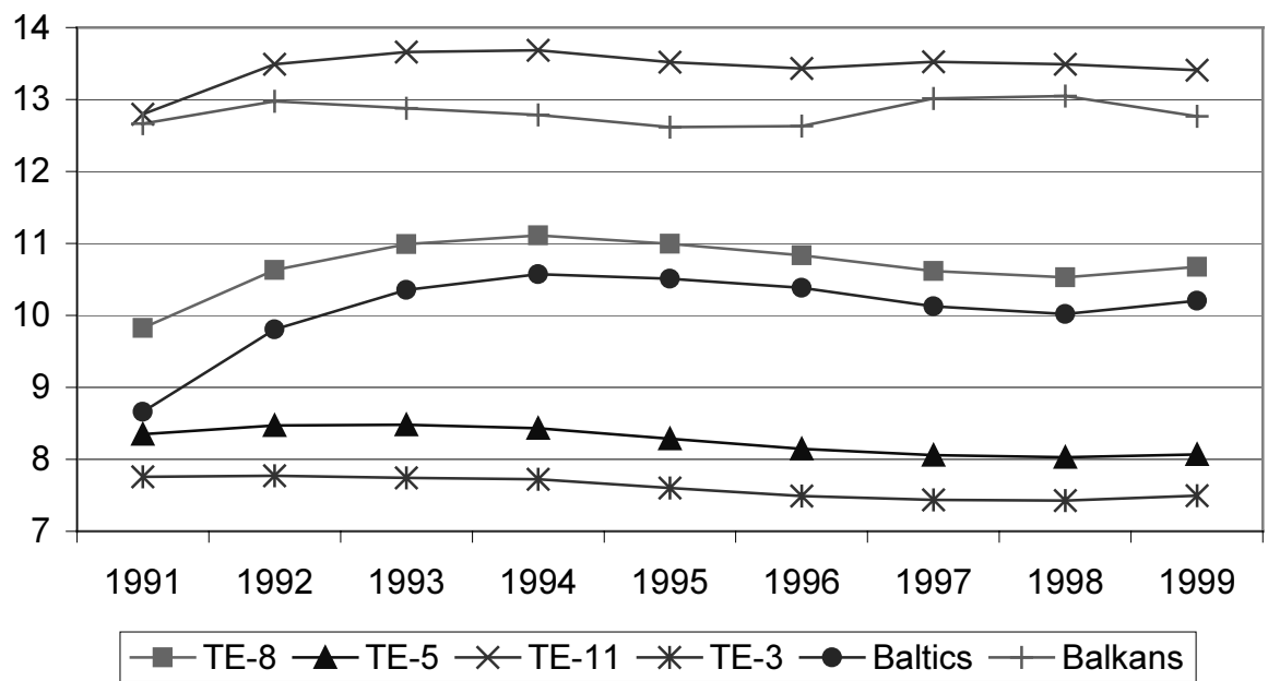
Figure 3. Coefficient of Variation, Standard Deviation over Mean
