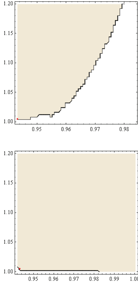
Figure 4: The top panel shows the domain of attraction for PLT with high credibility ( q_0^C = 0.9 ) and the bottom panels shows the domain for IT.
