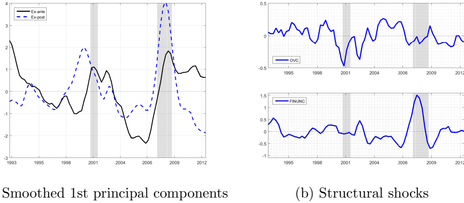
Figure 7: Principal components and shocks
