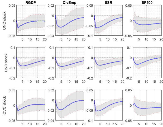
Figure 6: Uncertainty and overconfidence shock responses
