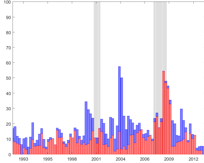
Figure A.3: Non-zero outer bins
