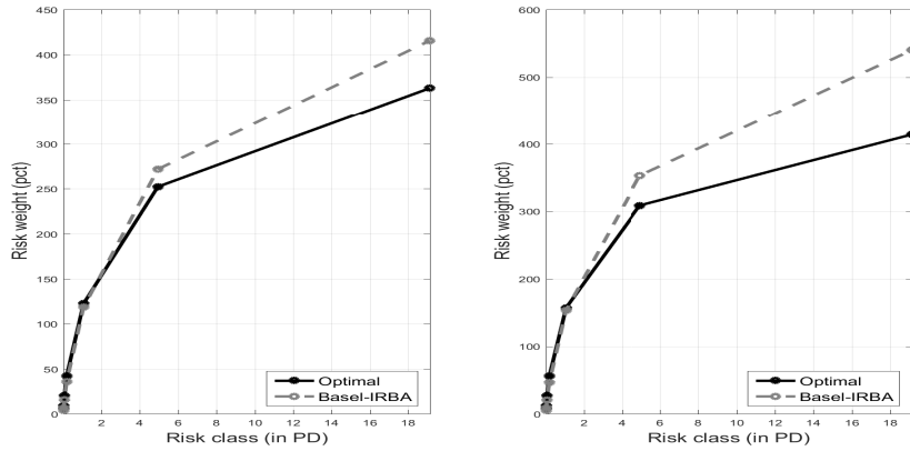
Figure 4: Risk weights: Optimal vs. Basel-IRBA
