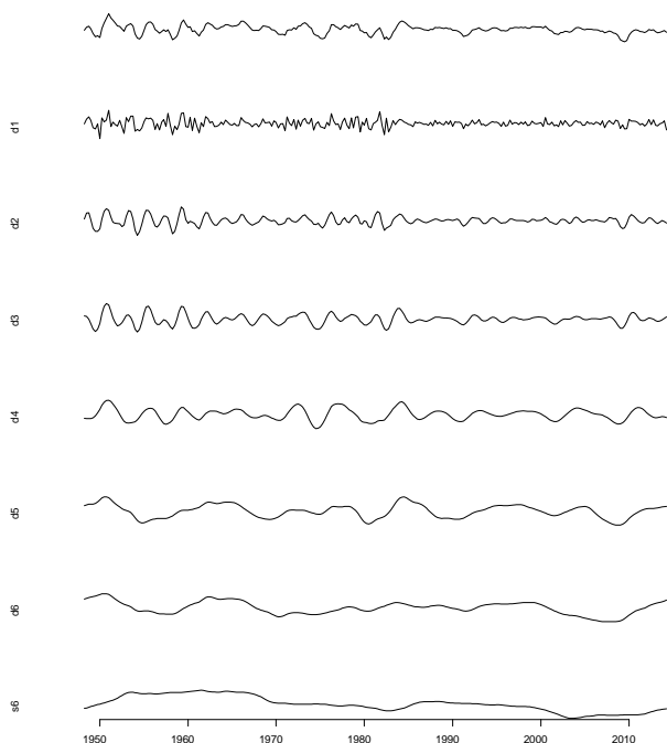
Figure 1: MODWT for log change US real GDP
