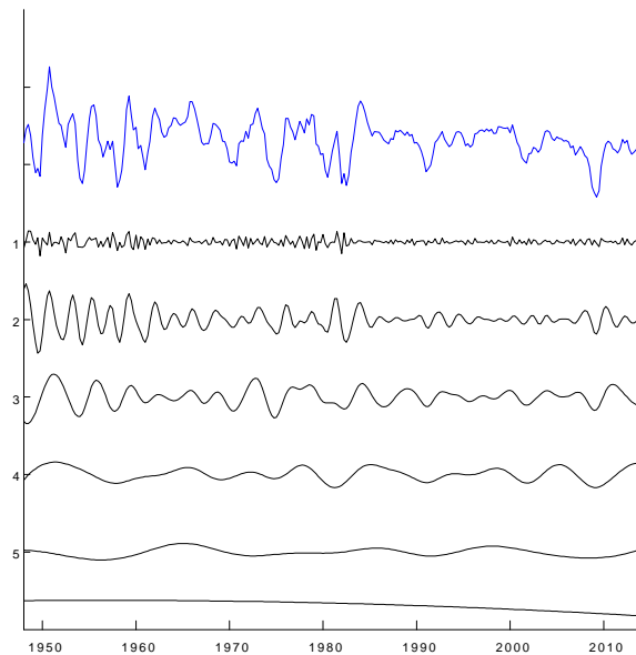
Figure 2: EEMD of log change US real GDP
