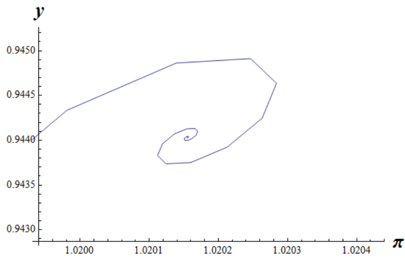
Figure 13: Initial \pi_t and y_t dynamics from near low steady state under PLT.
