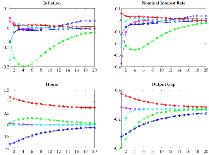
Figure 1: Impulse response functions - Reis (2009) model
