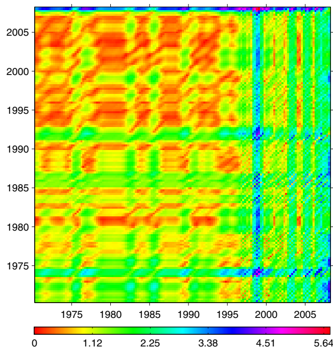
Figure 24: Unthresholded cross recurrence plot for Irish vs euro area growth rates.
