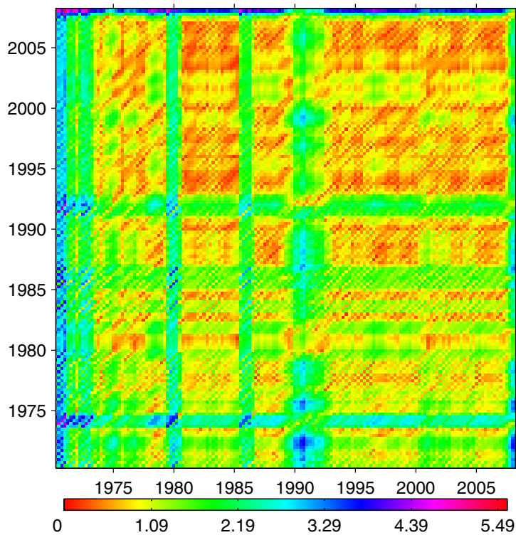
Figure 26: Unthresholded cross recurrence plot for Spanish vs euro area growth rates.
