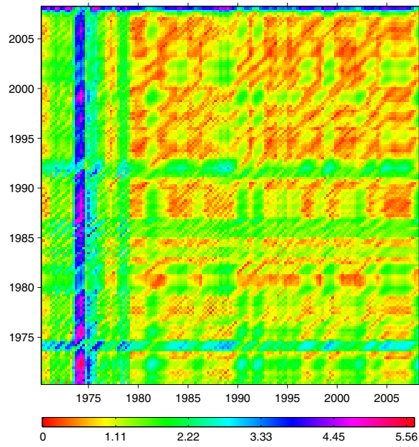
Figure 38: Unthresholded cross recurrence plot for Swiss vs euro area growth rates
