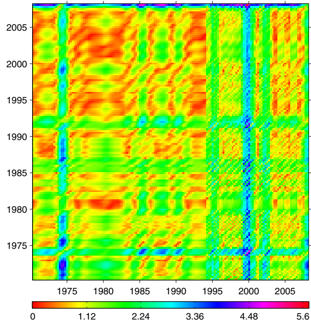
Figure 19: Unthresholded cross recurrence plot for Luxembourg vs euro area growth rates.
