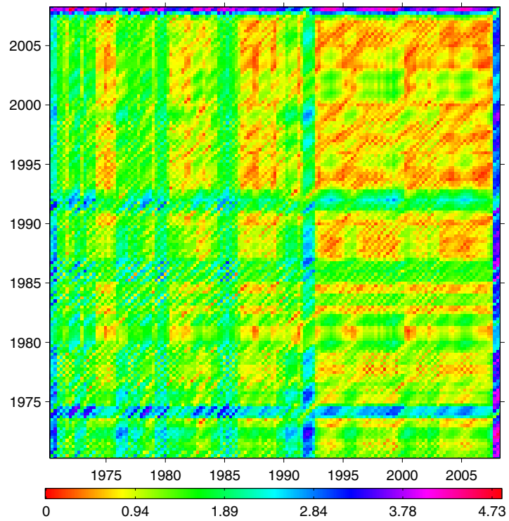
Figure 32: Unthresholded cross recurrence plot for Swedish vs euro area growth rates
