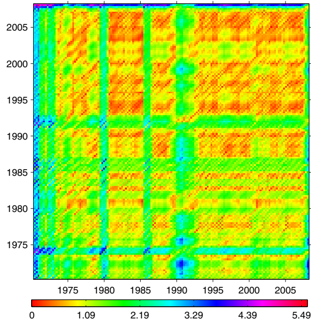
Figure 21: Unthresholded cross recurrence plot for Finnish vs euro area growth rates.
