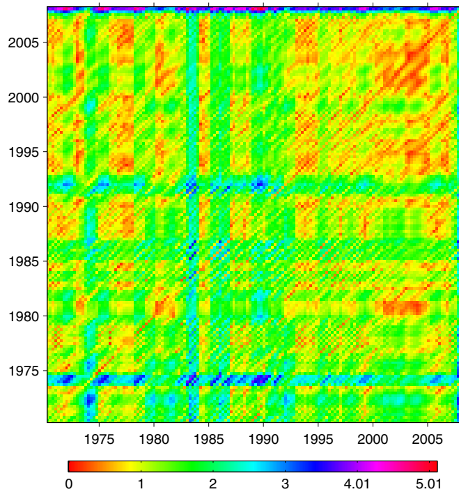
Figure 13: Unthresholded cross recurrence plot for German vs euro area growth rates.
