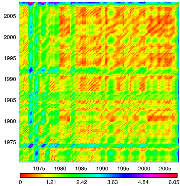
Figure 16: Unthresholded cross recurrence plot for Italian vs euro area growth rates.
