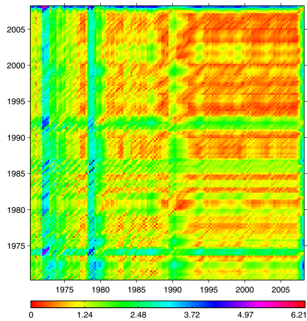
Figure 35: Unthresholded cross recurrence plot for UK vs euro area growth rates
