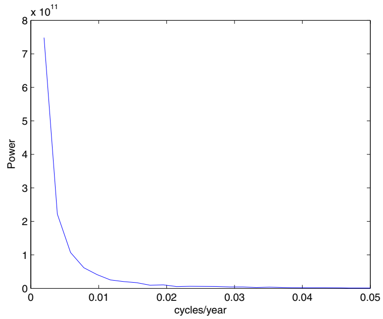
Figure 3: Periodogram for US real GNP level data
