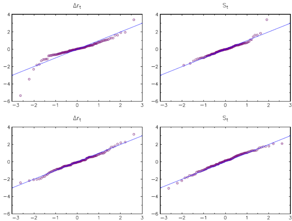
Figure 2: Quantile-quantile plots of the residuals of the VAR(3,0)- N (upper panel) and VAR(2,1)- t (lower panel) models for the US term structure data.
