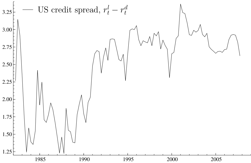
Figure 1: The raw US credit spread for the time period 1982:4–2007:4
