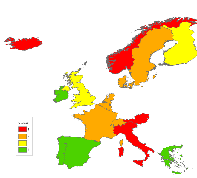
Figure 4: Cluster map for 1983–1991 vs Germany
