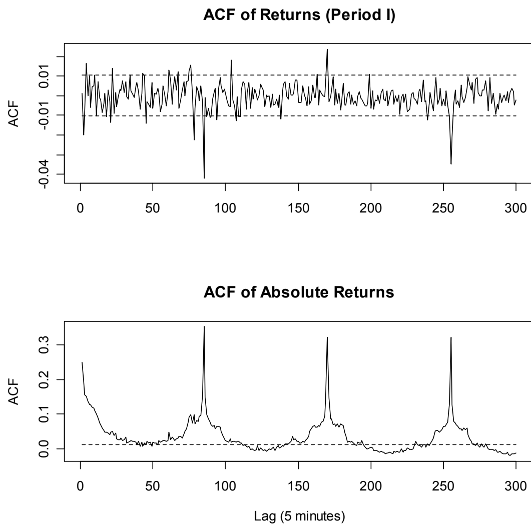
Figure 3: The sample ACFs of returns and absolute returns in Period I. The 95% confidence interval (dashed line) is for Gaussian white noise: \pm 1.96/\sqrt{N} .
