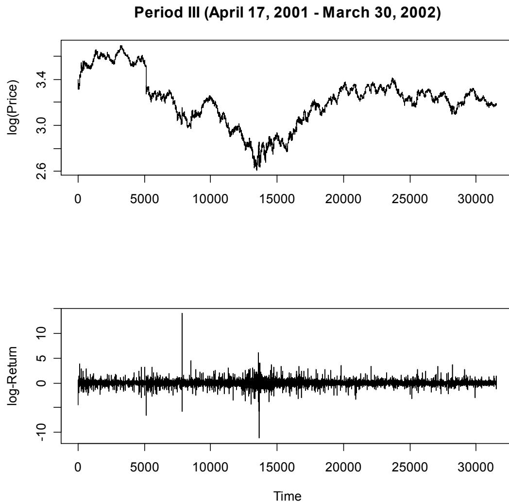
Figure 2: Price and return series of Period III (altermath period)
