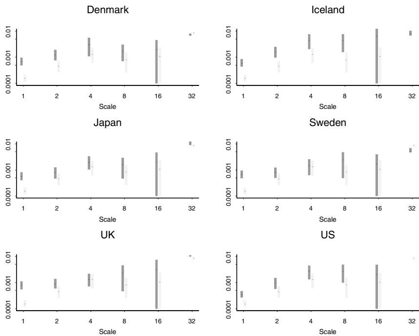
Figure 14: Wavelet variance: group 3
