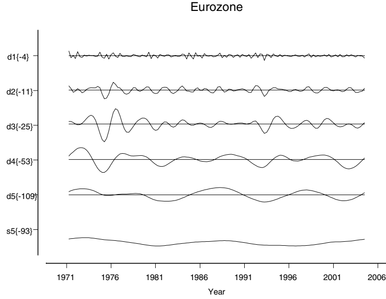
Figure 2: MODWT
