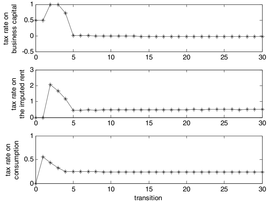
Figure 1: Optimal tax rates when \tau^n \geq 0 and \tau^k \leq 1 .
