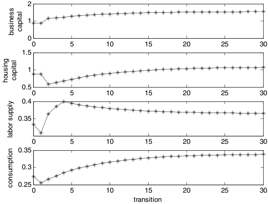
Figure 2: Transition paths when \tau^n \geq 0 and \tau^k \leq 1 .
