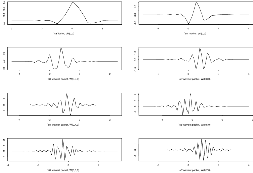
Figure 16: Debauchies wavelet packet functions
