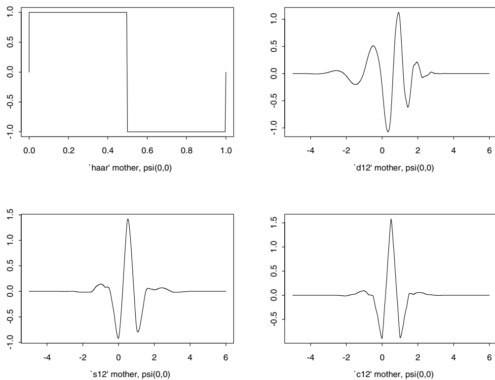
Figure 3: Families of wavelets
