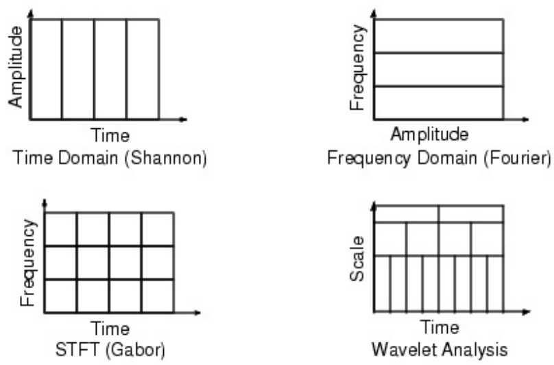
Figure 1: Fourier vs Wavelet analysis
