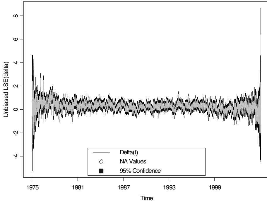
Figure 34: Instantaneous difference parameter estimates using LS for \text{abs}(\text{GBP/USD})
