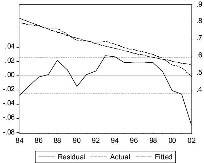
Logistic model: time series, fitting and residuals
